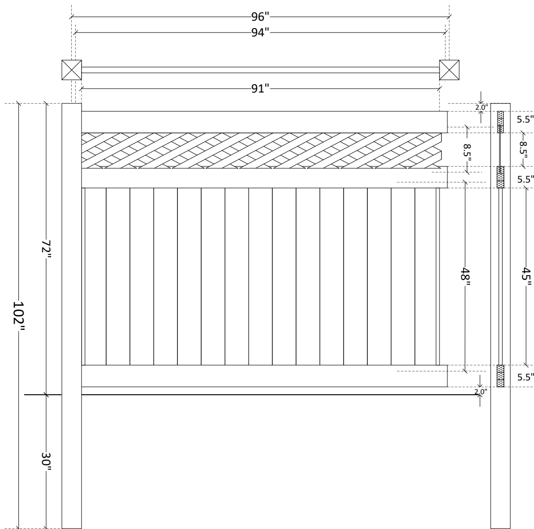
6' H X 8' Albemarle Privacy w/ Lattice
