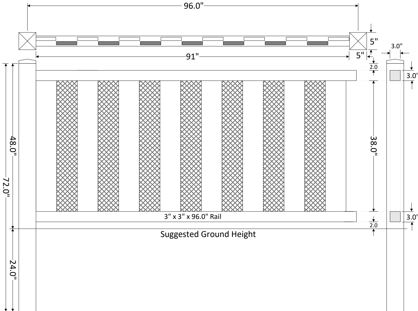
Hatteras (Shadow Box) Fence 4' H x 8' on Center
