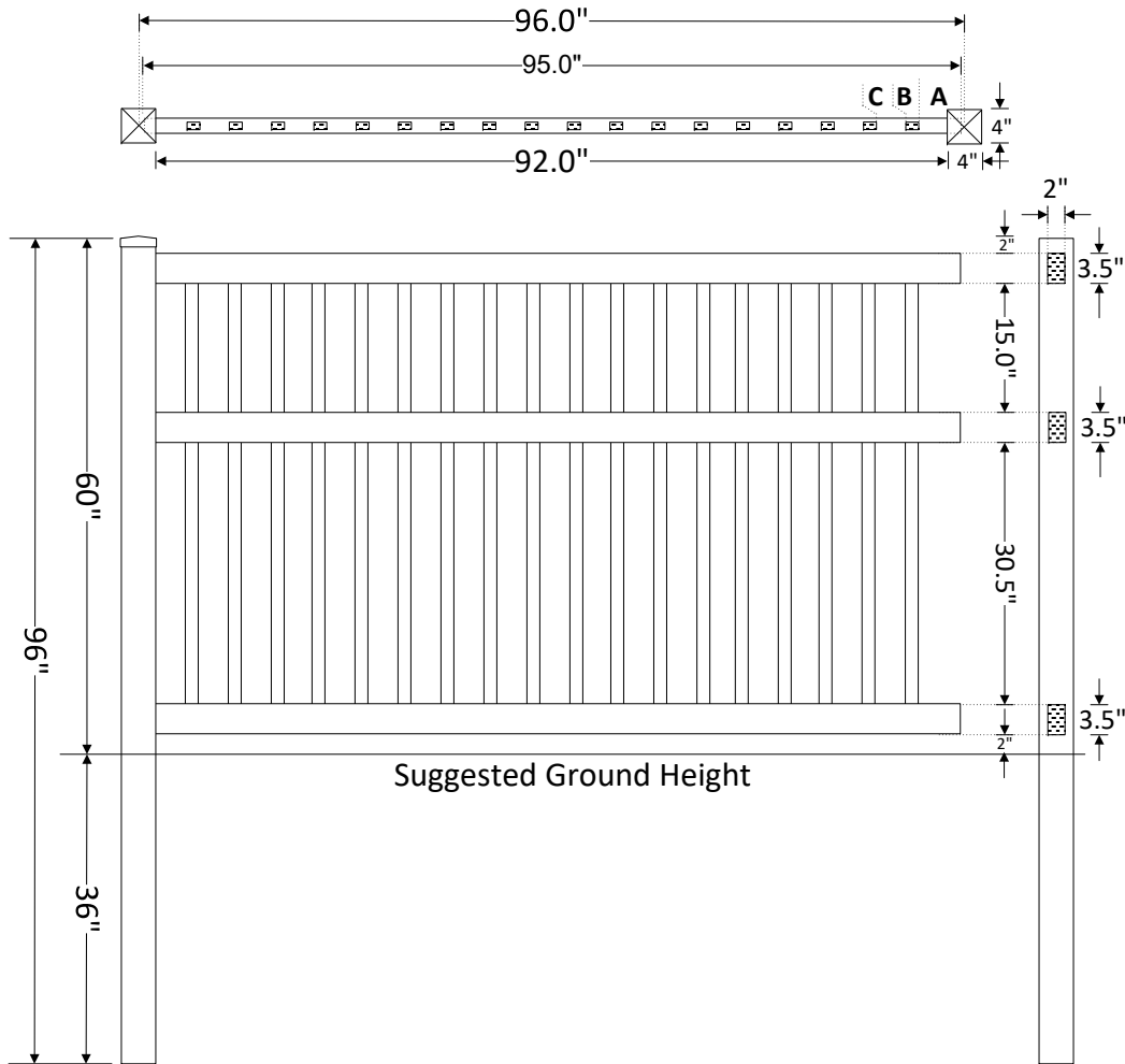
Myrtle Beach Fence 5' H x 8' on Center
