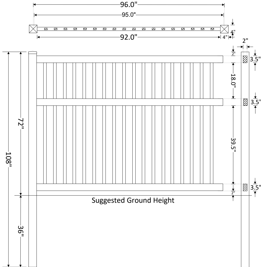
Myrtle Beach Fence 6' H x 8' on Center
