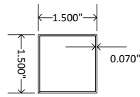
1.5" x 1.5" Square Picket
