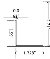
Aluminum J-Channel Insert (Top Rail)
